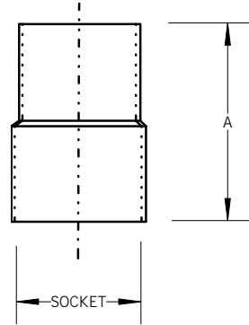
Flex Hose Adapter Hose Spigot x Duct Bell
