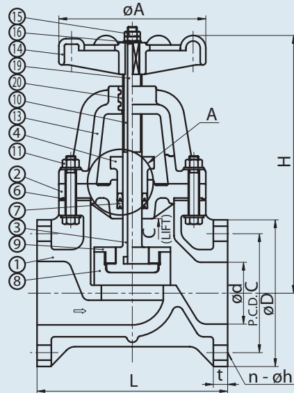
FLANGED 2 1/2" — 4"
