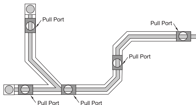
Figure D-34. Pull port locations for leak detection cable
