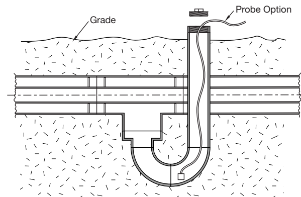
Figure D-37. In-line inspection well
