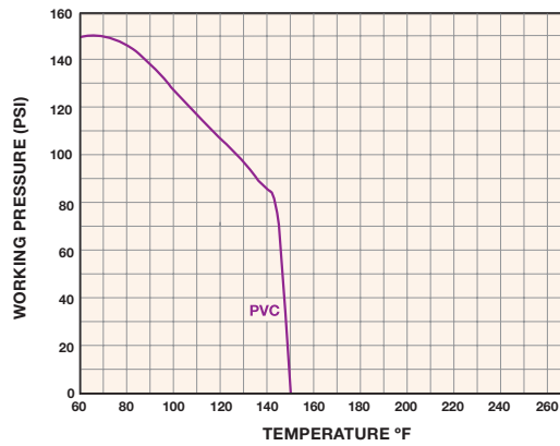
OPERATING TEMPERATURE/PRESSURE
